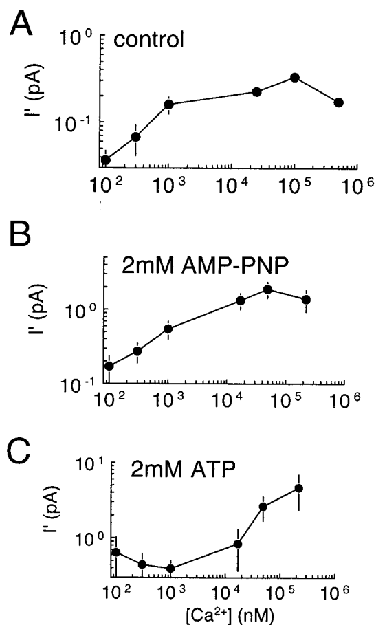
FIGURE 11 Cytoplasmic [\text{Ca}^{2+}] -sensitivity of RyRs is reduced by phosphorylation. Average mean current ( I' ) ( n = 5-8 RyR N channels) obtained over a range of cis [\text{Ca}^{2+}] under control conditions ( A ), in the presence of 2 mM cis AMP-PNP ( B ), and in the presence of 2 mM cis ATP ( C ). Note that the curve is shifted higher [\text{Ca}^{2+}] in the presence of ATP.
