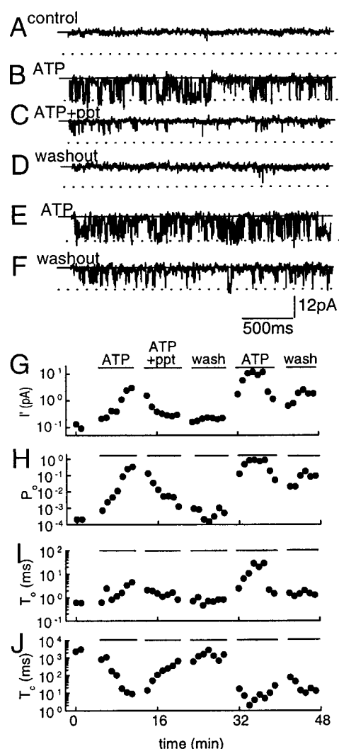
FIGURE 3 Acid phosphatase reduces activation of RyRs during prolonged exposure to ATP. Activity is shown from an \text{RyR}_\text{N} channel at -40 mV with 300 \text{ nM} cis \text{Ca}^{2+} . Channel opening is downward. A–F each show a 3-s recording of channel activity under control conditions ( A ), 5 min after addition of 2 \text{ mM} cis ATP ( B ), 5 min after addition of 10 units of acid phosphatase to the cis chamber ( C ), 4 min after perfusion of ATP from the cis chamber ( D ), 5 min after a second addition of 2 \text{ mM} cis ATP ( E ), and 5 min after reperfusion of the cis chamber ( F ). The history plots in G–J show average I' , P_o , T_o , and T_c measured during continuous 30-s recordings taken every minute during the experiment. The first two points were obtained under control conditions, then cis ATP was added (ATP) followed by phosphatase (ATP + ppt), ATP and phosphatase were washed out of the cis chamber (wash), ATP was then added alone to the cis chamber (ATP), and finally washed out (wash).
